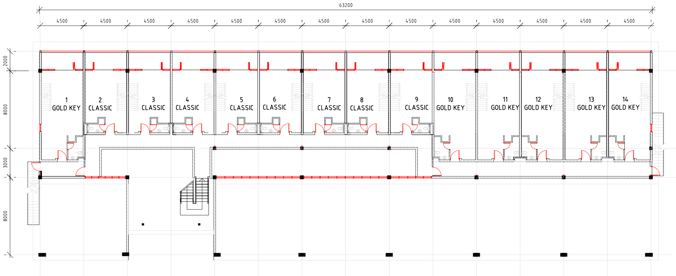
FIRST FLOOR PLAN SCALE 1 : 200
